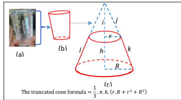
Figure 3. Truncated Cone Illustration
