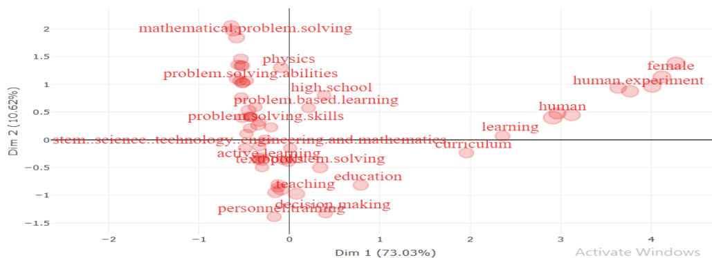
Figure 11. Factorial Analysis
