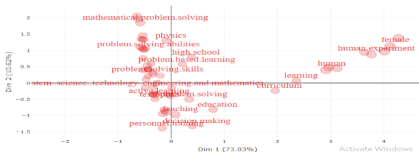
Figure 11. Factorial Analysis
