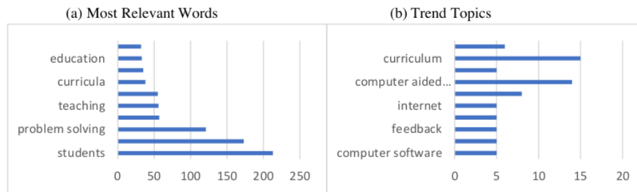
(c) WordCloud
